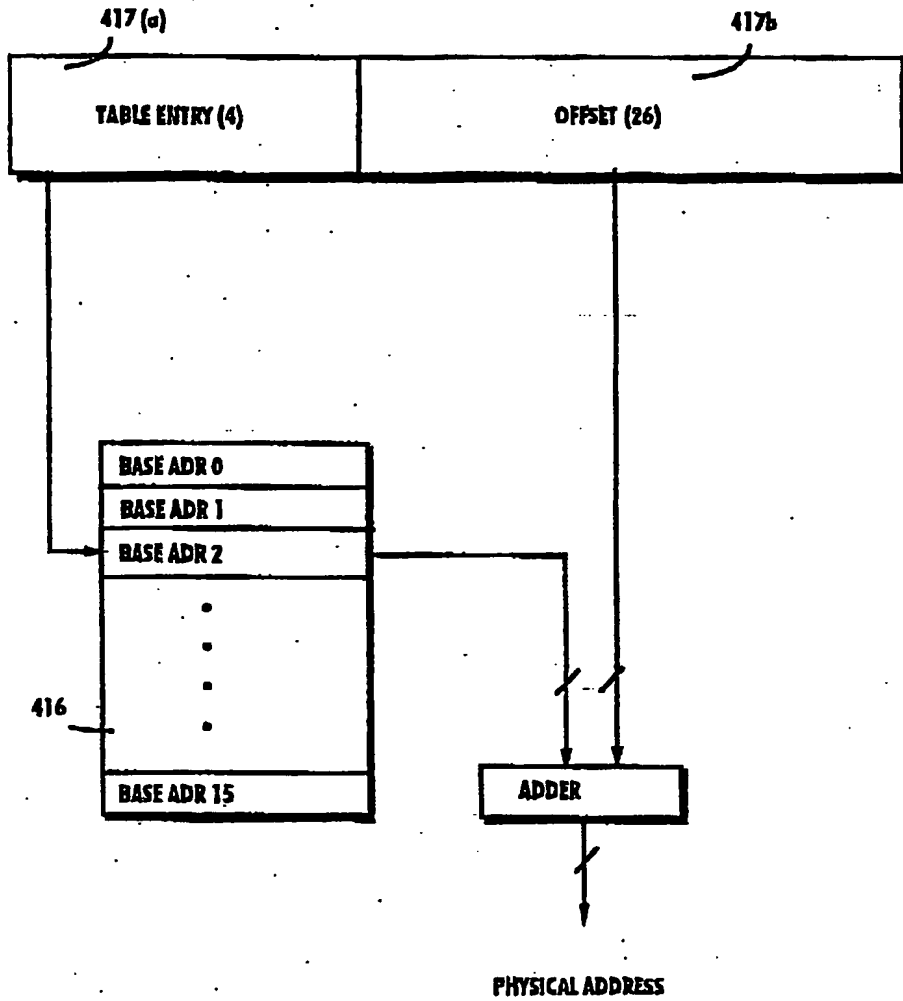
EXAMPLE SIGNAL PROCESSOR SEGMENT ADDRESSING
